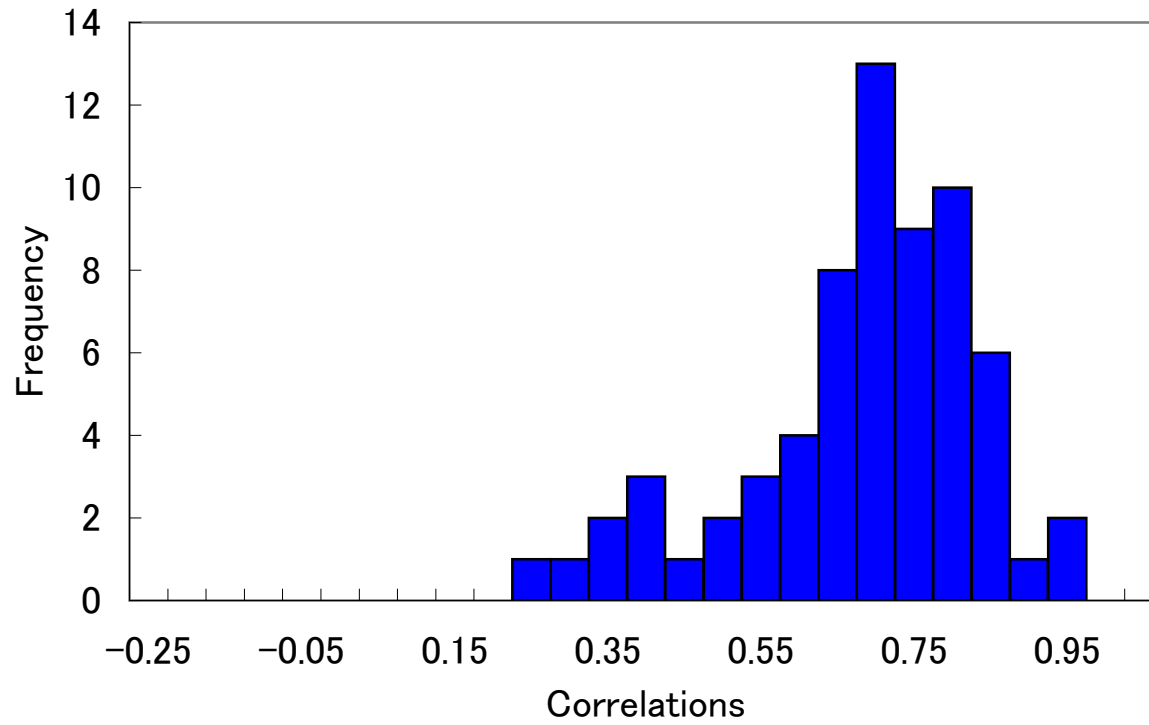
Figure 2: UK 12 Regions Cross-correlations
