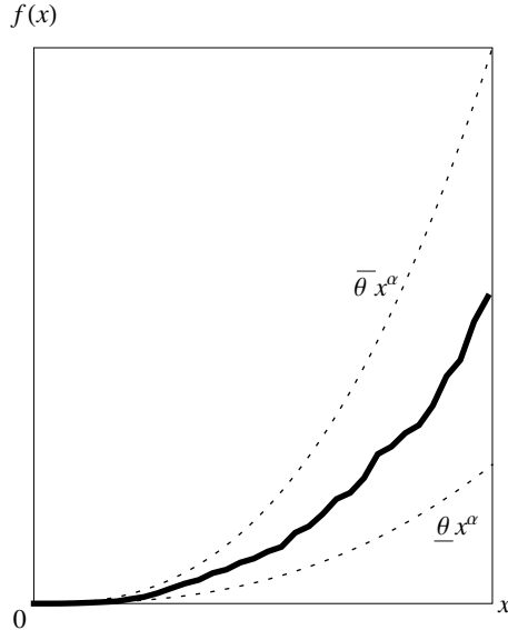
Figure 2: Production function of the form (4.8)
